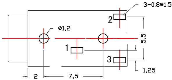
P. C. B TERMINAL POSITION
