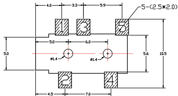
P. C. B TERMINAL POSITION
