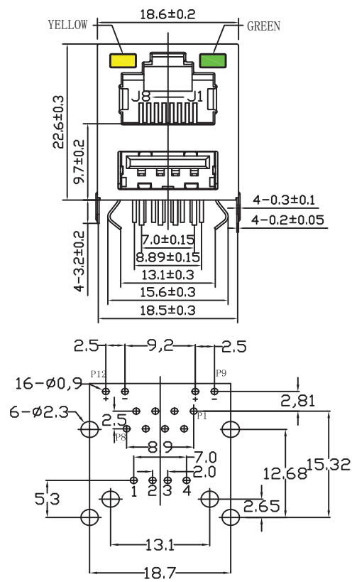
RECOMMEND PCB LAYOUT
